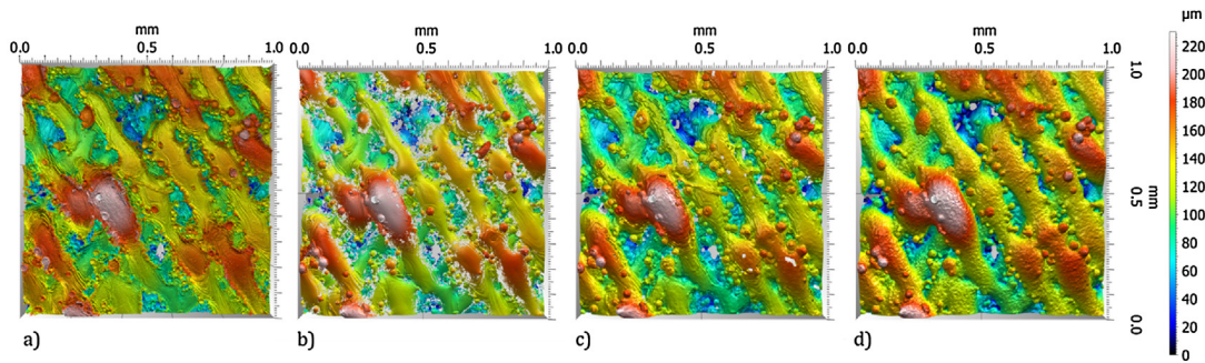
Fig. 1. Reconstructed portions of aligned topographies (top views, height-based colouring); (a) CM; (b) CSI; (c) FV; (d) XCT.
