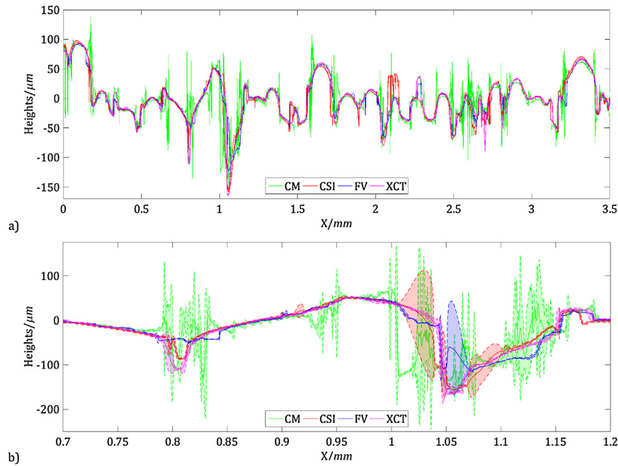
Fig. 2. Profile comparison; (a) twelve profiles (three for each instrument) obtained from cross-sectioning along the diagonal of the (2.5 × 2.5) mm aligned topographies; (b) portion of the same cross-section: mean profiles and estimated CIs.
