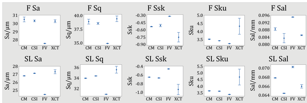
Fig. 3. CIs for the texture parameters computed on the F and SL sets.
