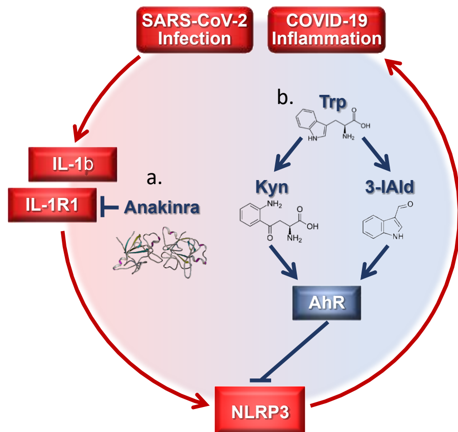
Figure 1. Targeting inflammatory pathways in coronavirus disease-19 (COVID-19) by tryptophan (trp) metabolites and Anakinra. (a) Anakinra inhibits NLRP3 by blocking IL-1R1 activation; (b) endogenous trp metabolites target AhR downregulating the NLRP3 pathway. Kyn = kynurenine; 3-IAld = Indole-3-carboxaldehyde.
