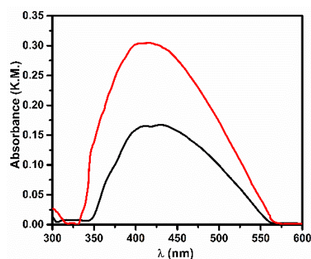
Figure 1. UV-Vis extinction spectra (Kubelka–Munk units) of SiO 2 -Ag before (black line) and after (red line) the 366 nm radiation.
