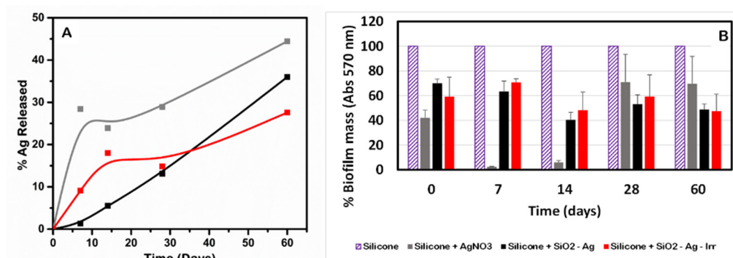
Figure 4. (A) Silver release from silicone functionalized with AgNO 3 (grey line), SiO 2 -Ag (black line) and SiO 2 -Ag-Irr (red line) in function of time. (B) Biofilm mass growth of A. niger in presence of silicone discs (purple striped columns) and functionalized silicone with AgNO 3 (grey columns), SiO 2 -Ag (black columns) and SiO 2 -Ag-Irr (red columns).
