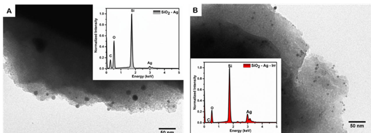
Figure 2. TEM images of SiO 2 -Ag (A) and SiO 2 -Ag-Irr (B). Insertion: EDX spectra of: (A) SiO 2 -Ag; (B) SiO 2 -Ag-Irr.
