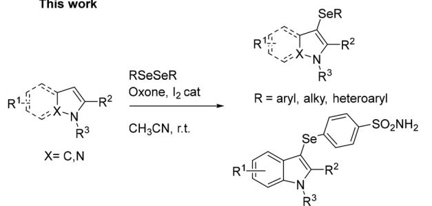
Fig. 2 Different strategies for the synthesis of 3-selenylindoles.
