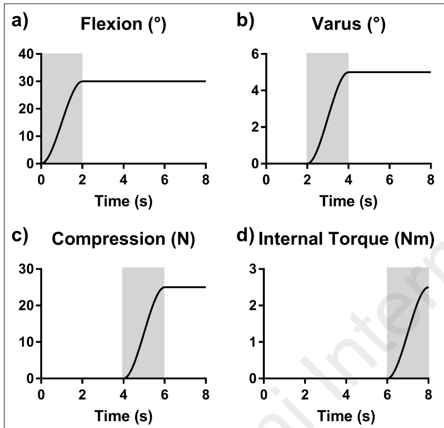
Figure 5 a-d. Loads and displacements applied to the forearm in the dislocation maneuver: a) flexion of the forearm from full extension ( 0^\circ ) to the set angle ( 30^\circ , 60^\circ or 90^\circ ); b) varus motion in the frontal plane from 0^\circ to 5^\circ ; c) compression force along the ulnar axis (from 0 to 10 N or 25 N); d) internal rotation torque around the ulnar axis (from 0 to 2.5 Nm).
