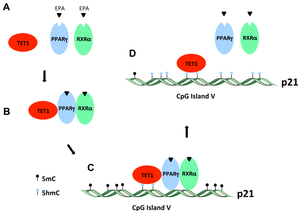
Figure 5. Schema of the EPA role in increasing 5hmC in the hypermethylated CpG island V on the p21 gene. A, B) EPA simultaneously bound PPAR \gamma and RXR \alpha receptors ( A ) to form their heterodimer and induced a PPAR \gamma -TET1 interaction ( B ). C) The TET1-PPAR \gamma -RXR \alpha protein complex bound to the CpG island V on the p21 gene where TET1 converted 5mC to 5hmC. D) TET1 associated stably to DNA, whereas PPAR \gamma and RXR \alpha exited, breaking up their heterodimer and EPA binding.
